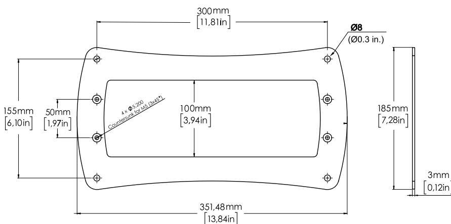
Figure 5: i-5 mounting bracket
