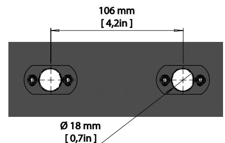
Figure 2: i-5 Series locking points
