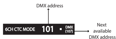
Figure 13: Set/edit DMX address
