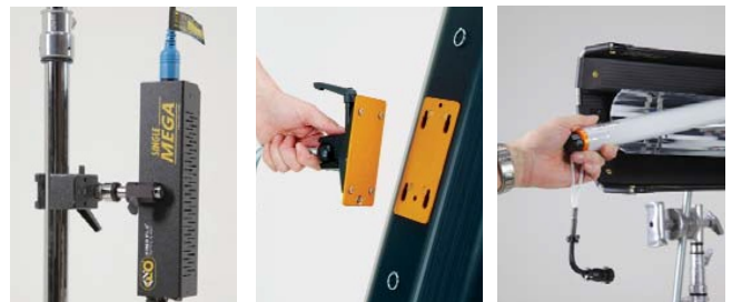
MTP-BAL Kino Ballast Baby Mount (16mm)
